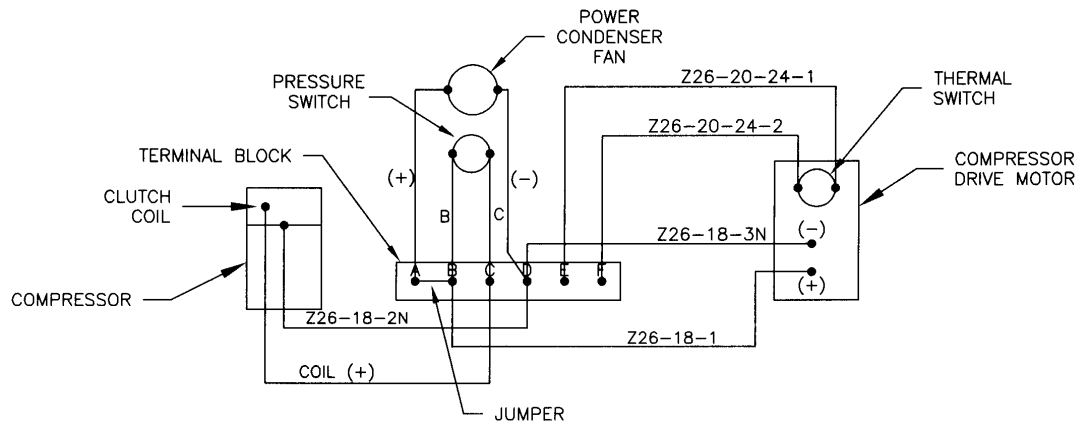
WIRING DIAGRAM 2.
