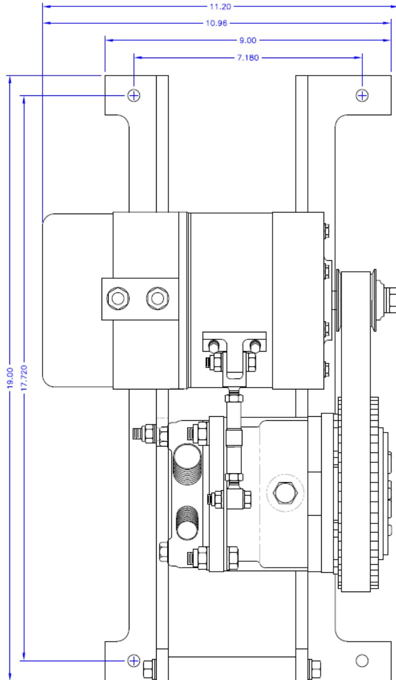
Z26-8900-6 ILLUSTRATION 4.
