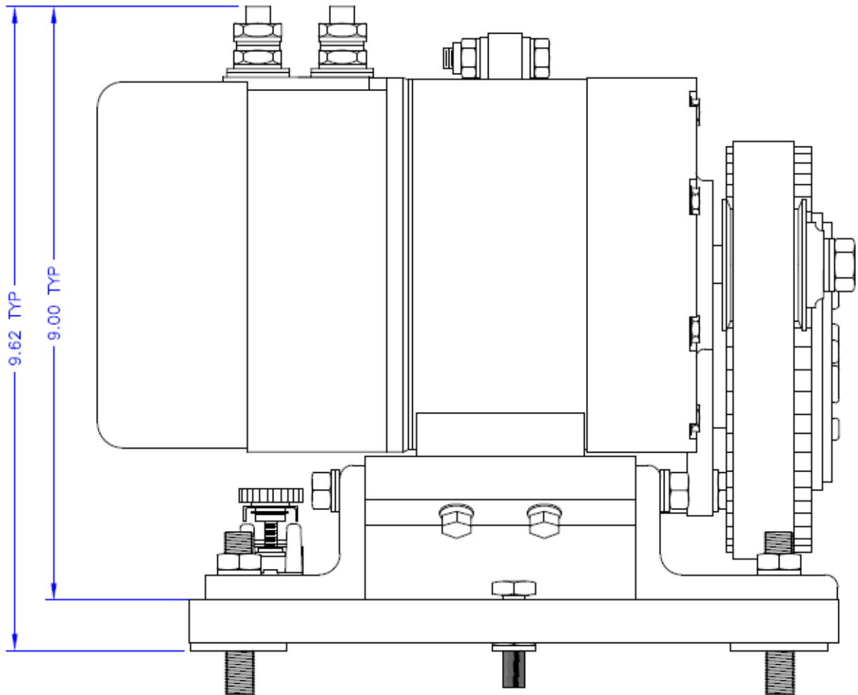
Z26-8900-7 / -8 / -9 ILLUSTRATION 5.
