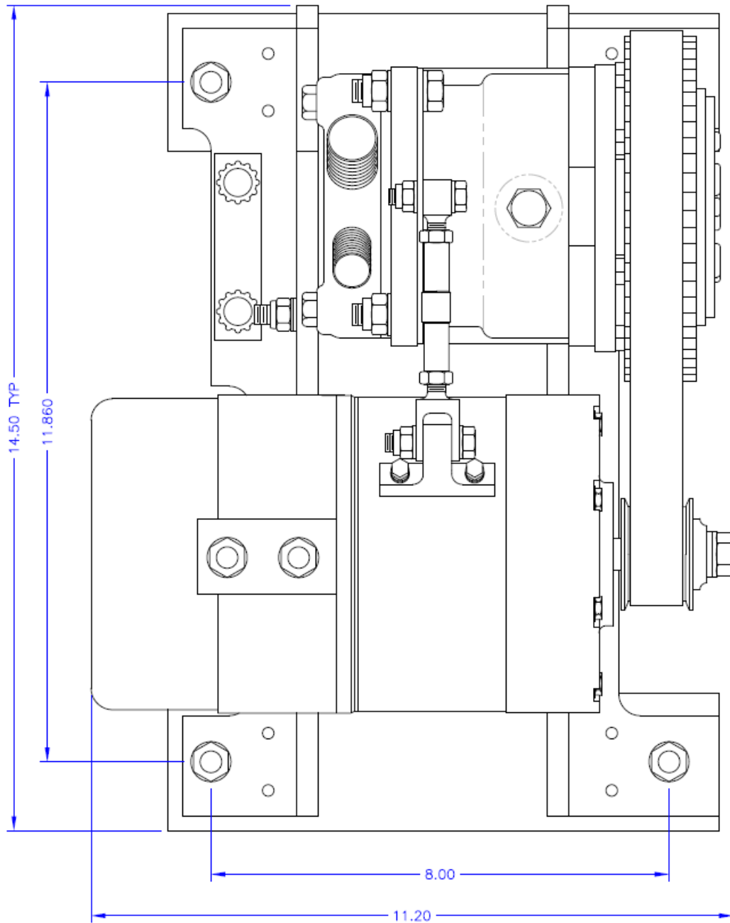
Z26-8900-7 / -8 / -9 ILLUSTRATION 6.
