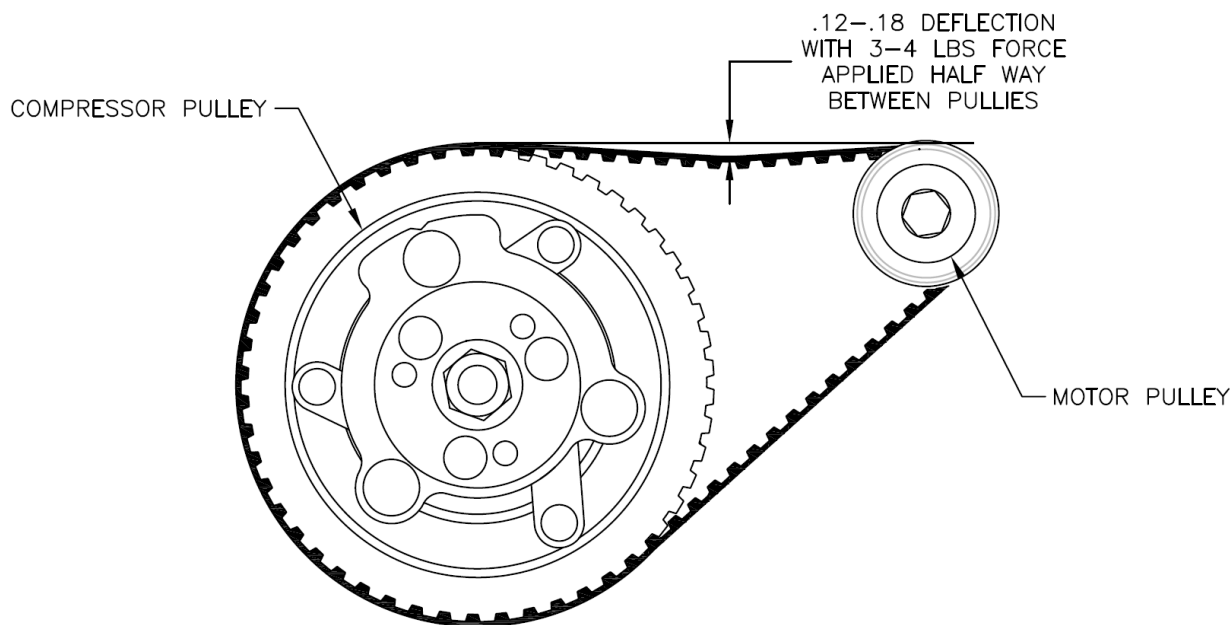
ILLUSTRATION 8.
