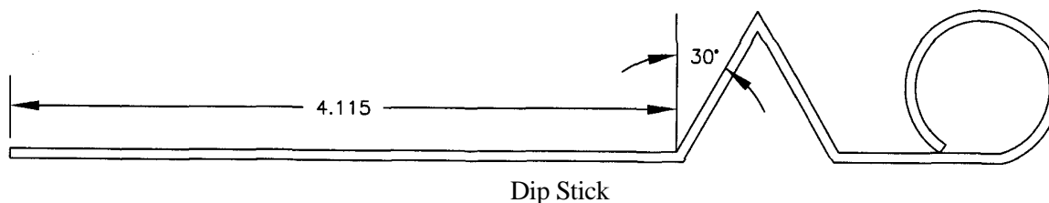
ILLUSTRATION 9.
