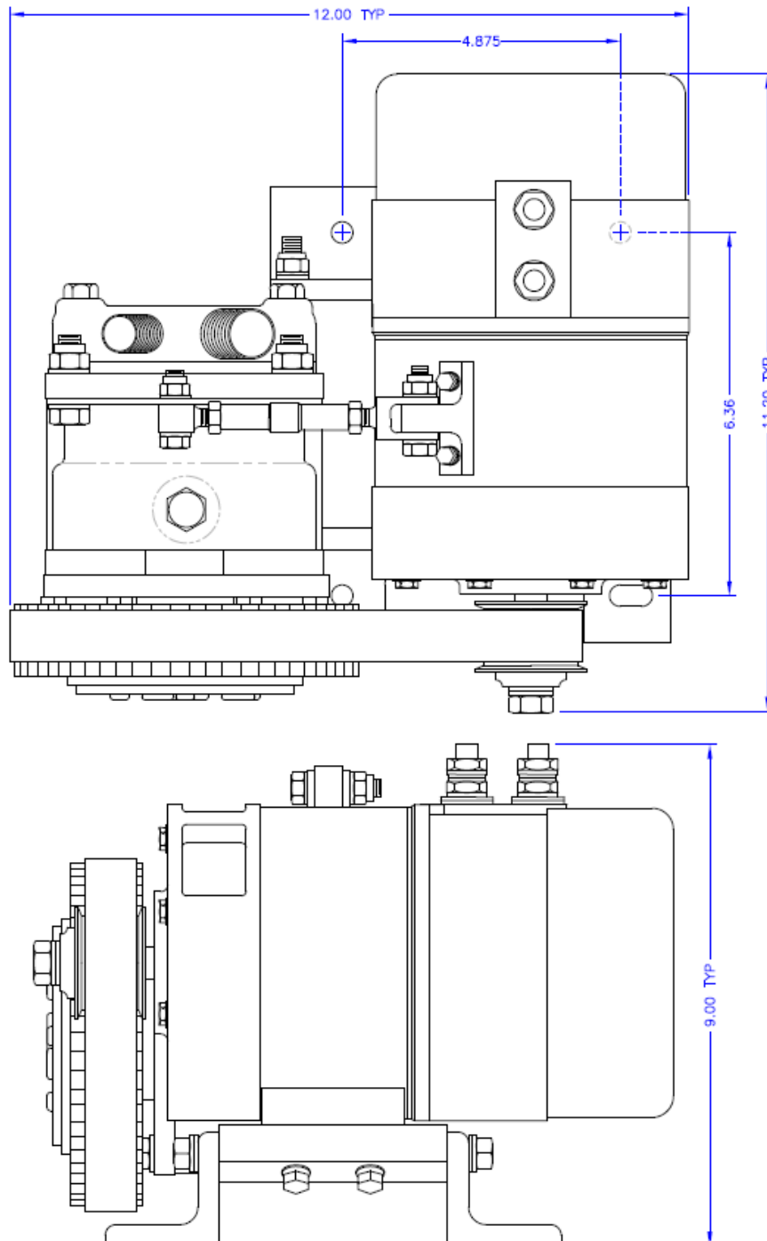
Z26-8900-2 / -4 ILLUSTRATION 2.
