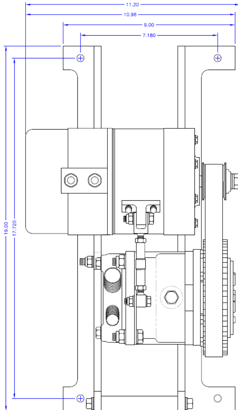
Z26-8900-6 ILLUSTRATION 4.
