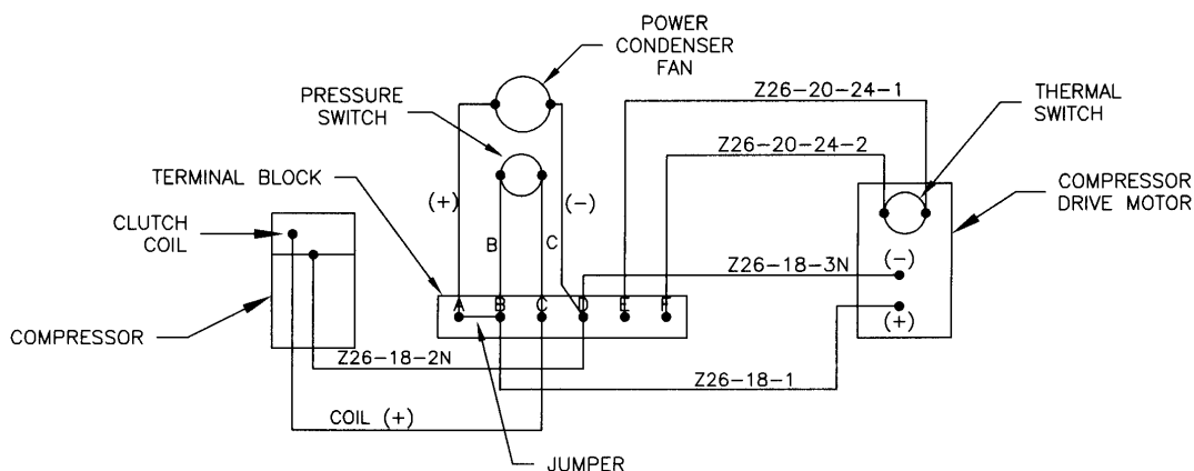
WIRING DIAGRAM 2.
