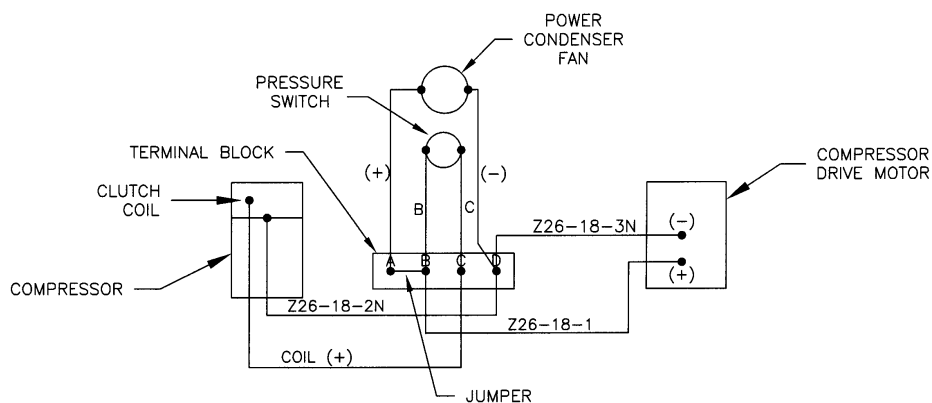
WIRING DIAGRAM 1.
