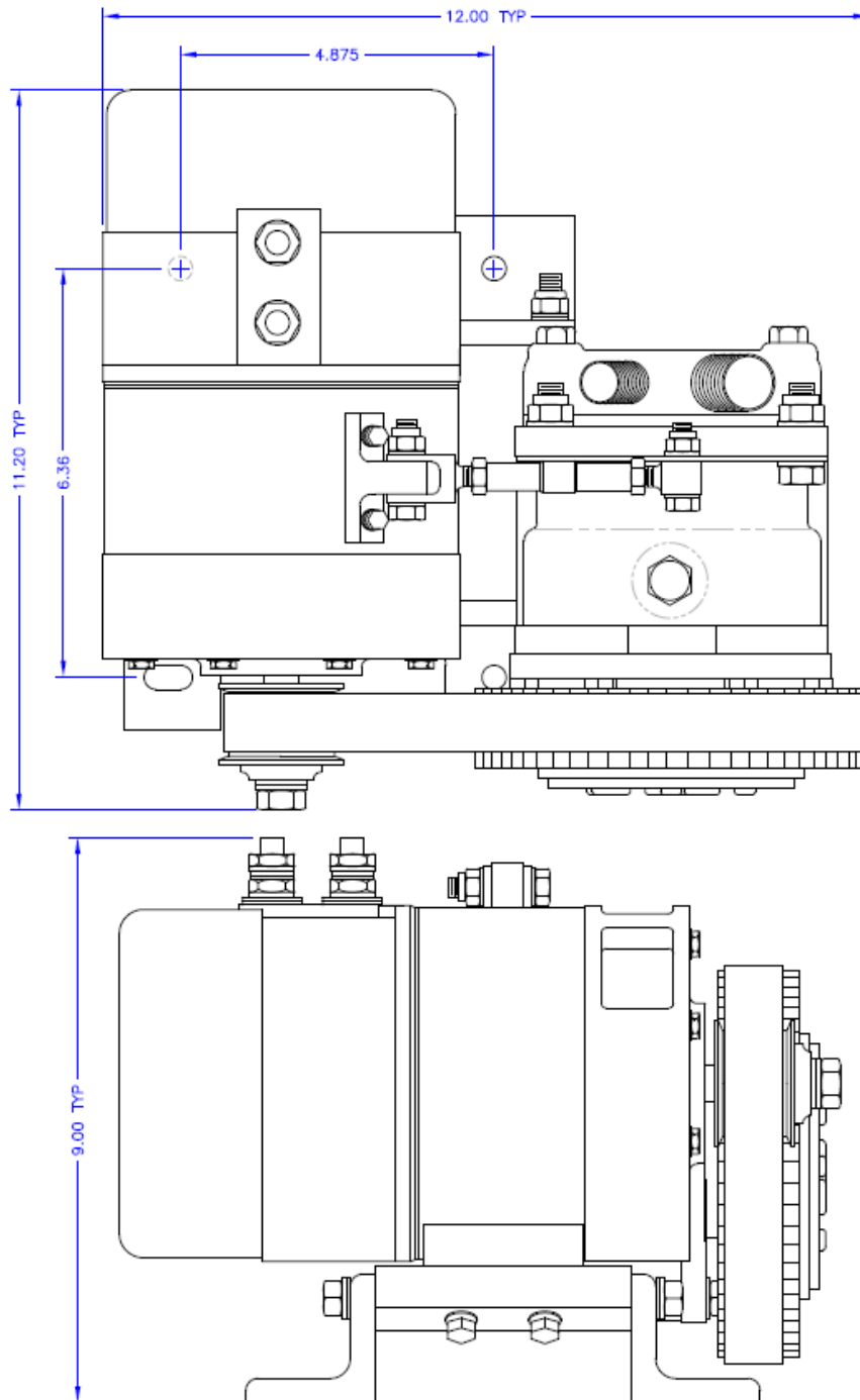
Z26-8900-1 / -3 / -5 ILLUSTRATION 1.
