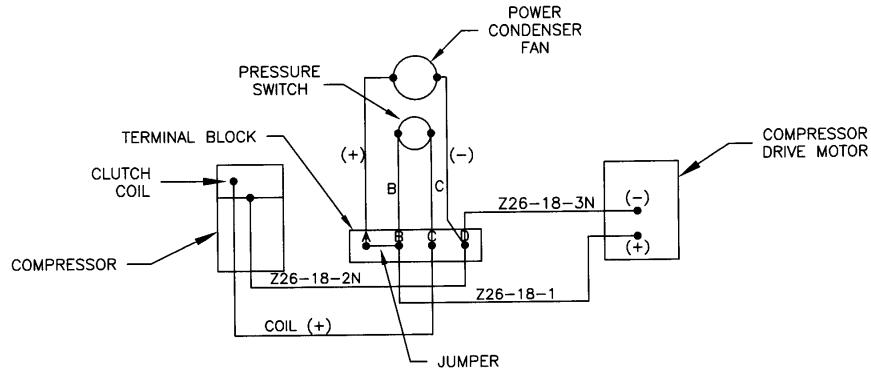
WIRING DIAGRAM 1.
