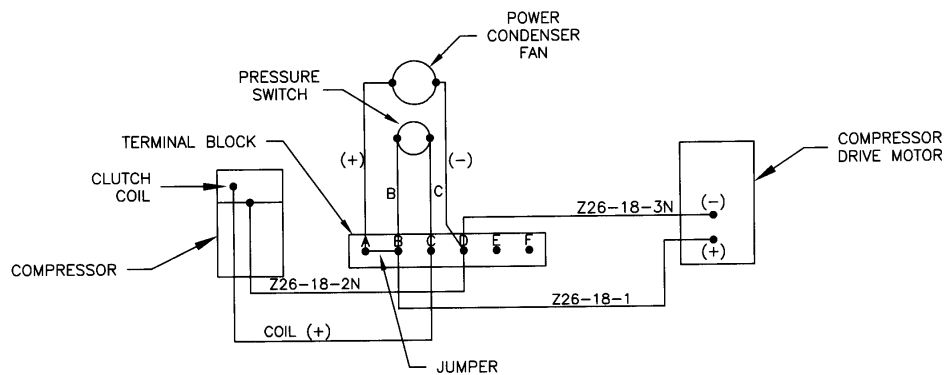
WIRING DIAGRAM 3.
