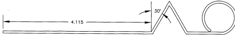
Dip Stick ILLUSTRATION 3.
