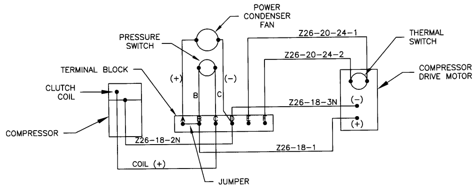
WIRING DIAGRAM 2.
